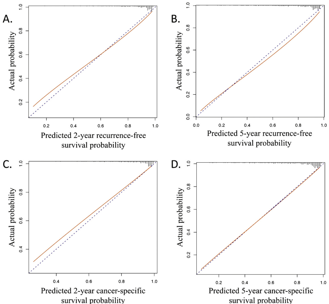
Fig. 2 – Calibration plots demonstrating the relationship between the nomogram-predicted 2- and 5-yr (A,B) recurrence-free (RFS) and (C,D) cancer-specific survival (CSS) probabilities and the observed survival probabilities in the external validation cohort. The solid line represents actual nomogram performance while the dotted line represents perfect calibration. AJCC = American Joint Committee on Cancer.
