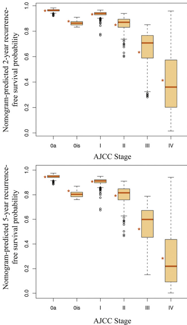
Fig. 3 – Box plots showing range of predicted recurrence-free survival (RFS) probabilities in the external validation cohort at 2 and 5 yr stratified by American Joint Committee on Cancer (AJCC) stage. The bold line indicates median, boxes represent the interquartile range (IQR), top whisker is upper quartile +1.5 \times IQR, and the bottom whisker is lower quartile -1.5 \times IQR. The red asterisks denote the predictions of each AJCC stage.
