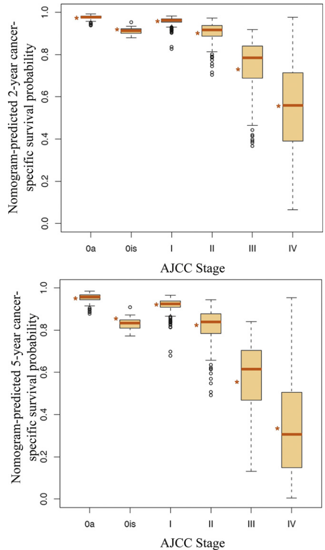
Fig. 4 – Box plots showing range of predicted cancer-specific survival (CSS) probabilities in the external validation cohort at 2 and 5 yr stratified by American Joint Committee on Cancer (AJCC) stage. The bold line indicates median, boxes represent the interquartile range (IQR), top whisker is upper quartile +1.5 \times IQR, and the bottom whisker is lower quartile -1.5 \times IQR. The red asterisks denote the predictions of each AJCC stage.
